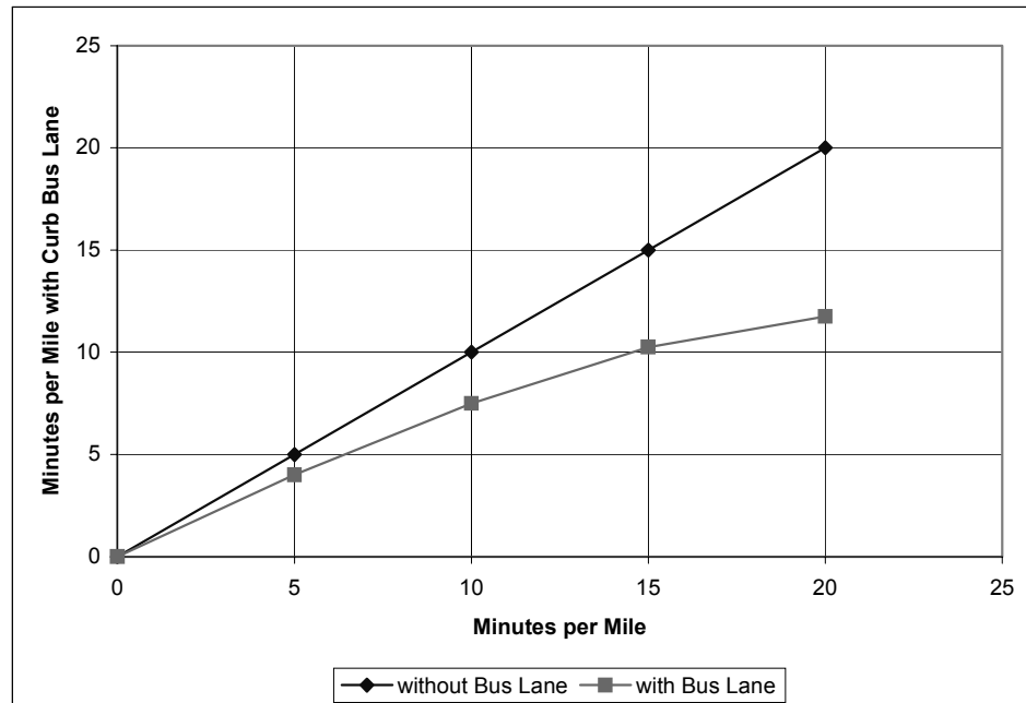
EXHIBIT 4-32 Time Savings with Curb Bus Lane
